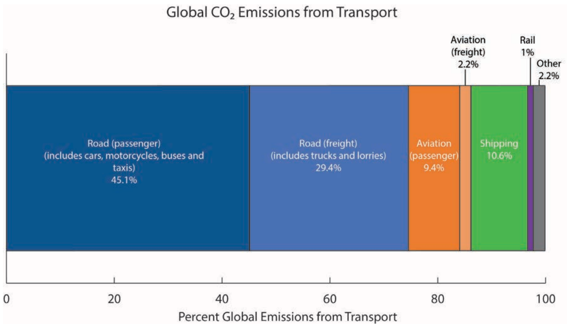
Figure 5.4 Global emissions from transportation sources 2
